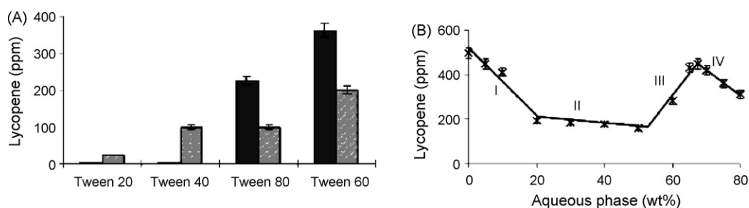
Fig. 3. Solubilization capacity in microemulsions as a function of surfactant type and aqueous dilution. (A) represents the solubilization capacity of lycopene in microemulsions of composition (1, solid bars) (R)-(+)-limonene/ethanol/Tween 60® (1:1:3) and 75% aqueous phase and (2, hatched bars) limonene/ethanol/Tween 60® (1:1:8) and 75% aqueous phase. (B) represents lycopene solubilization as a function of aqueous weight percent in the microemulsions in relation to the structural transition regions of the microemulsion (Spernath et al., 2002).
